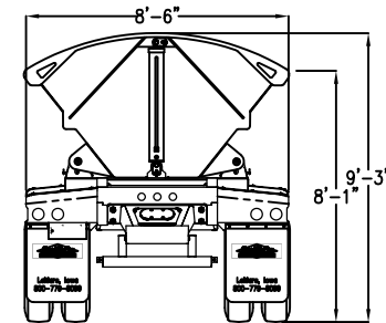
V-Shaped Tub
