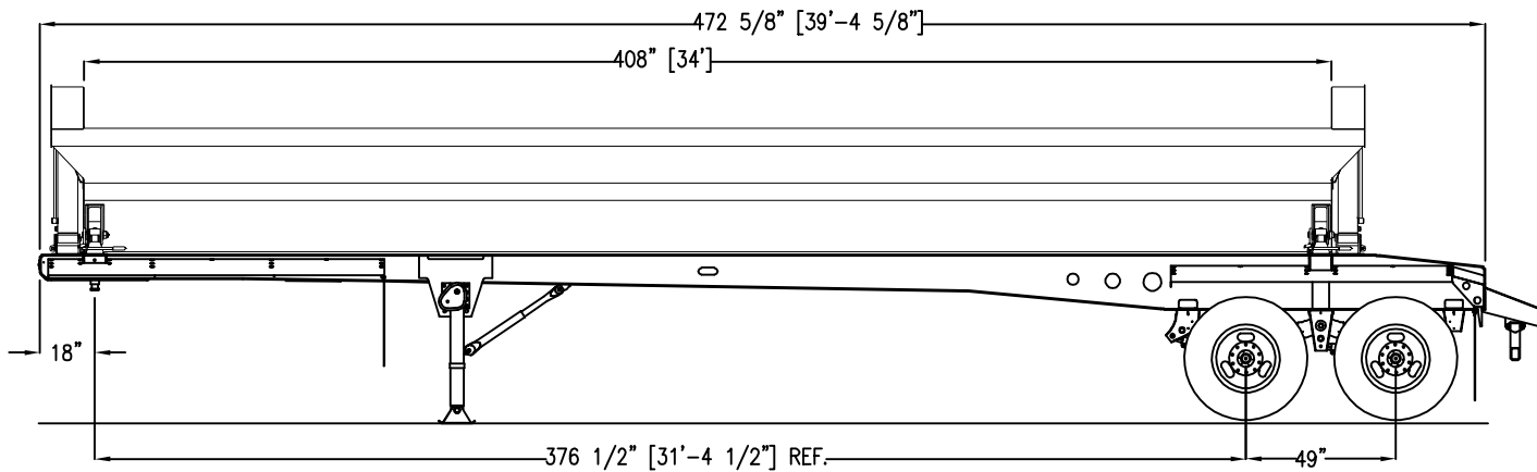
Model S2-4034 SmithCo Side-Dump Trailer
