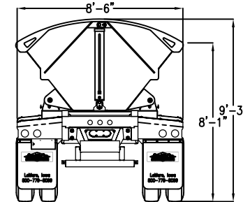
V-Shaped Tub
